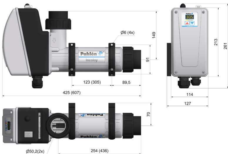
Dimensions for 12 - 15kW within brackets
